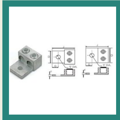
Aluminum Double Barrel Connector One Hole Mount
